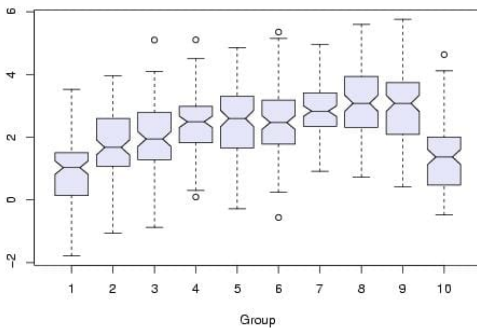
Notched Boxplots
